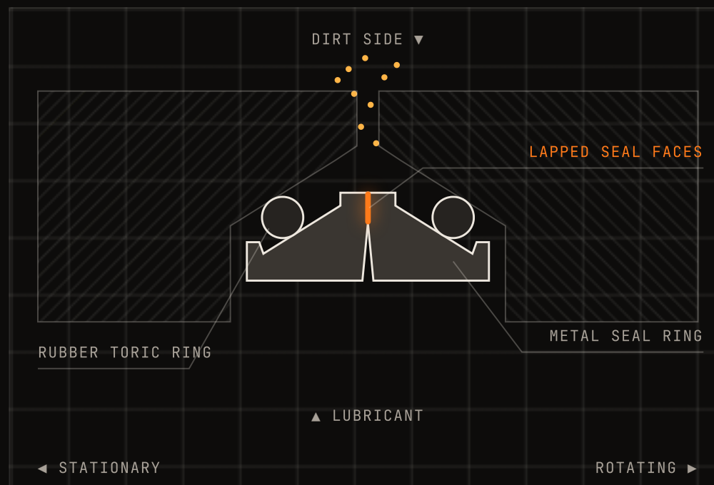
TORIC-LOADED METAL FACE SEAL
