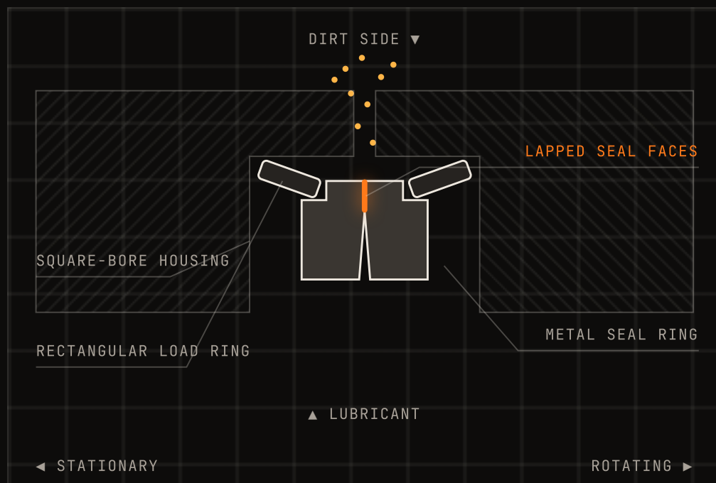
HEAVY DUTY DUAL FACE
